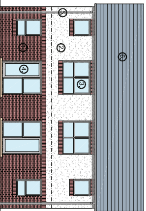
REAR ELEVATION (1:100)
