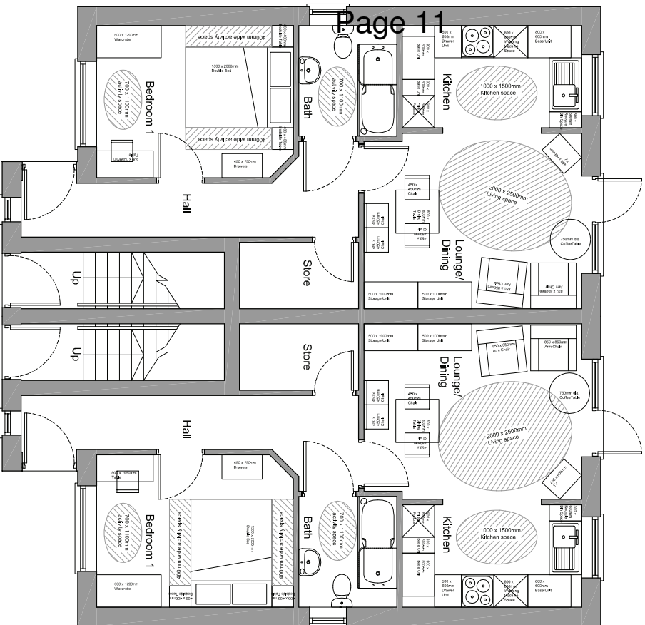
GROUND FLOOR (1:50) Type A (45.2m² / 486sq.ft.)
