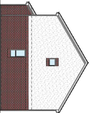
SIDE ELEVATION (1:100)
