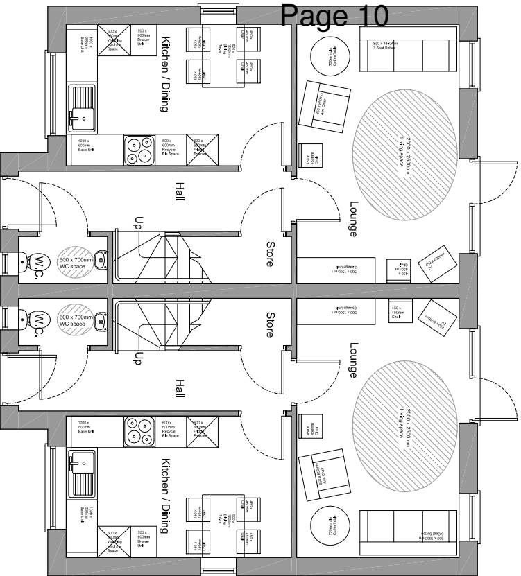
GROUND FLOOR (1:50) Type C (76.2m² / 820sq.ft.)
