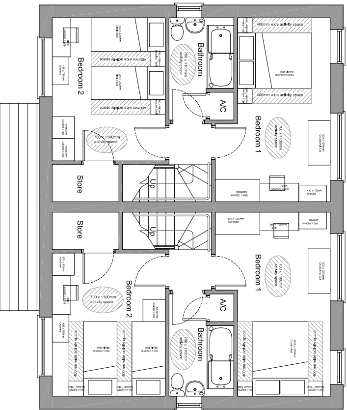
FIRST FLOOR (1:50)
